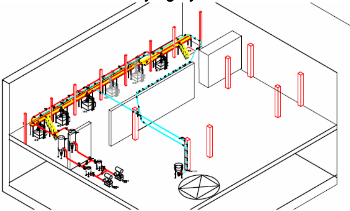
Soap Chip Loading System
