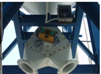
Diverter Valve
