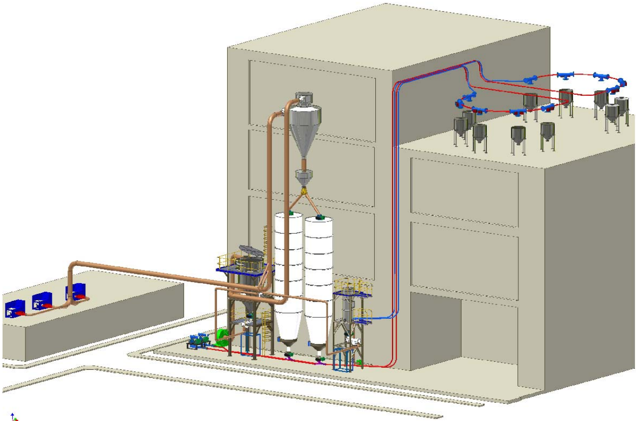
Pulp Chip Conveying System , (Raw material for dynamite manufacturing)
